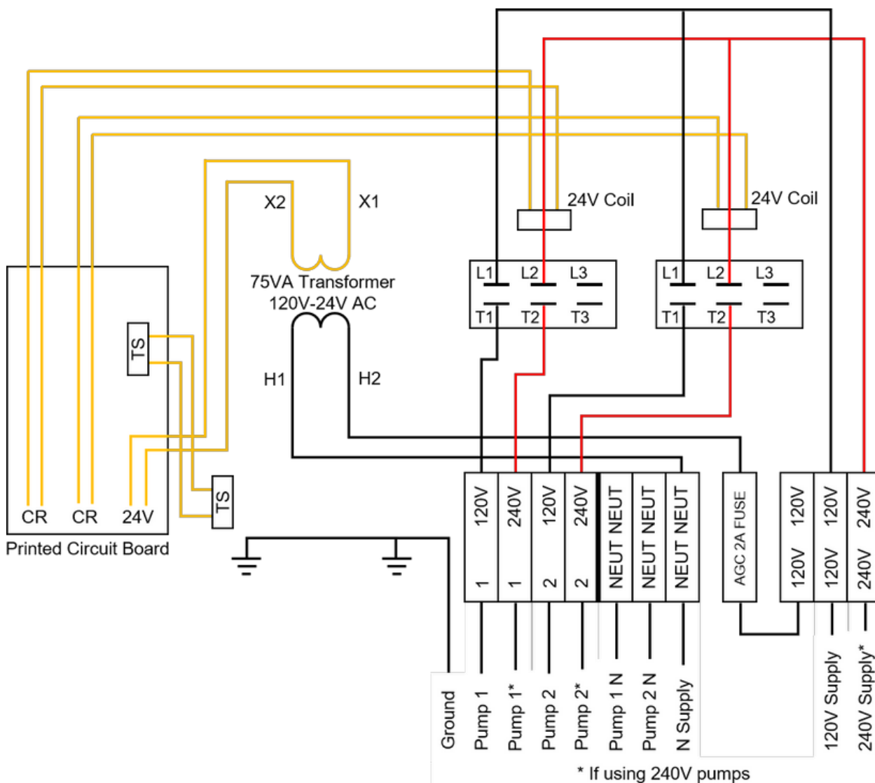
Figure 8: Fuel Lock Device Schematic Wiring Diagram
