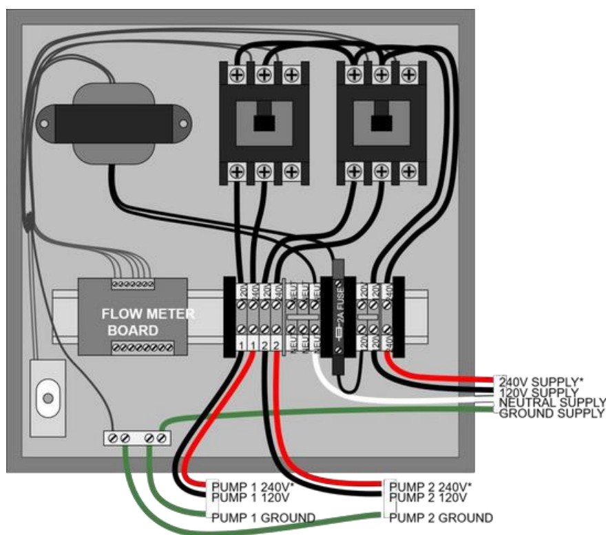
Figure 7: Fuel Lock 240v Pump Wiring
