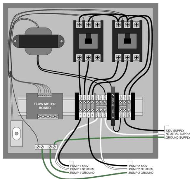
Figure 6: Fuel Lock 120V Pump Wiring
