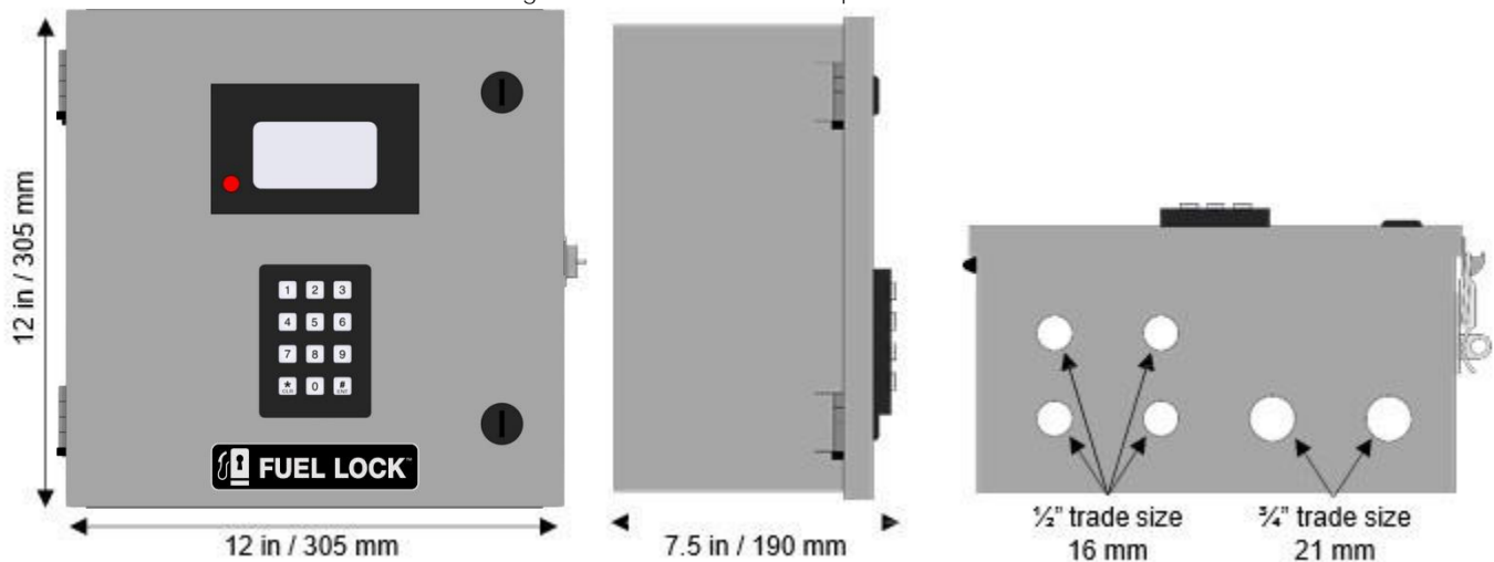
Figure 2: Fuel Lock Device Specifications
