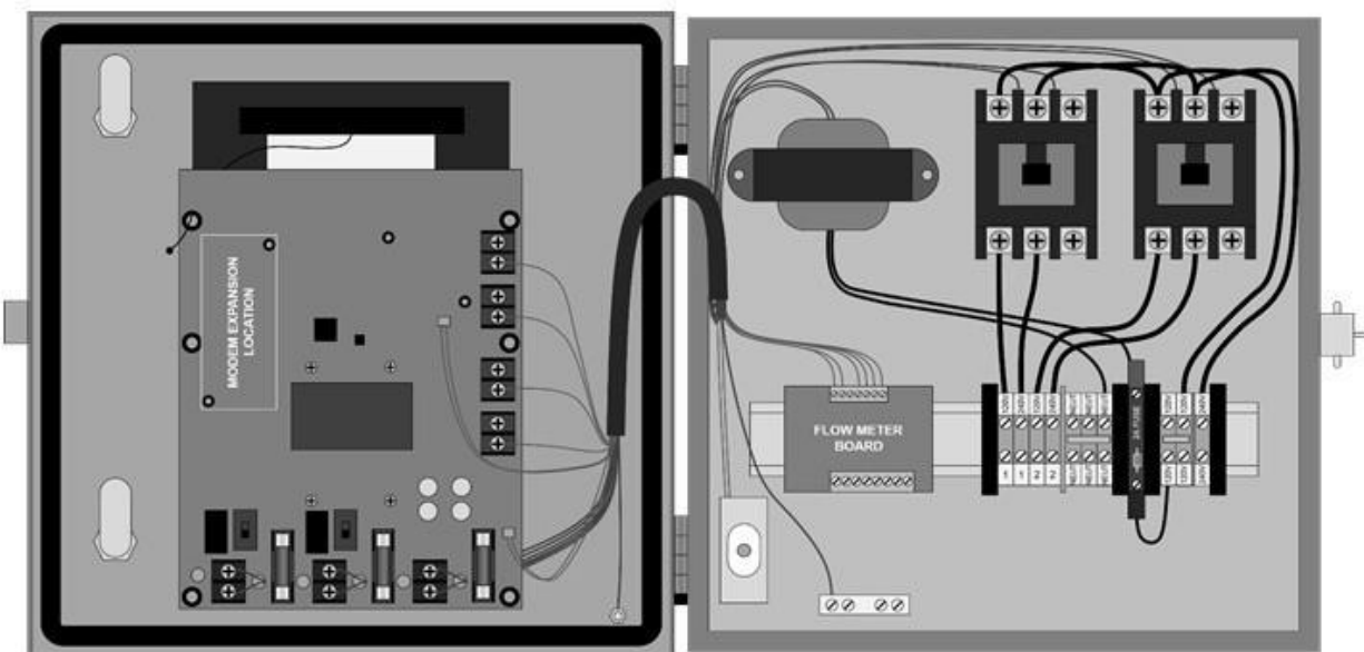
Figure 3: Fuel Lock Device (inside view)
